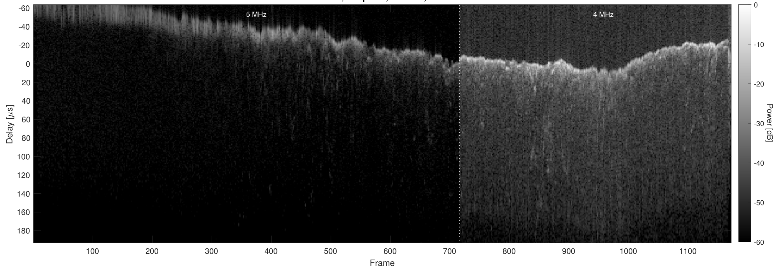
Orbit 17702, Chapman, Window, Channel 2
