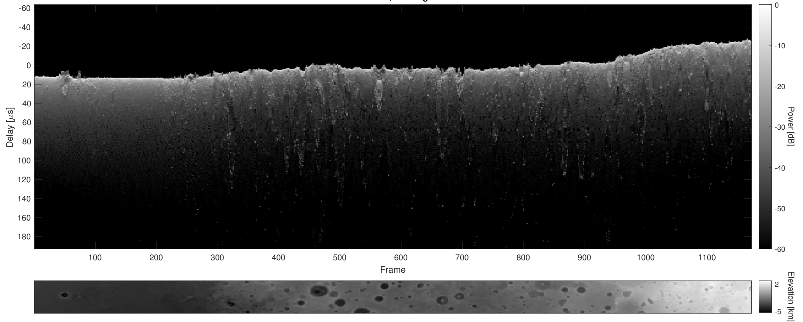
Orbit 17702, Cluttergram
