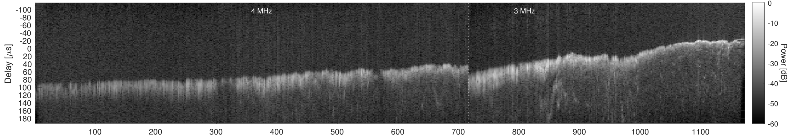
Orbit 17702, Window, Channel 2, Chapman
