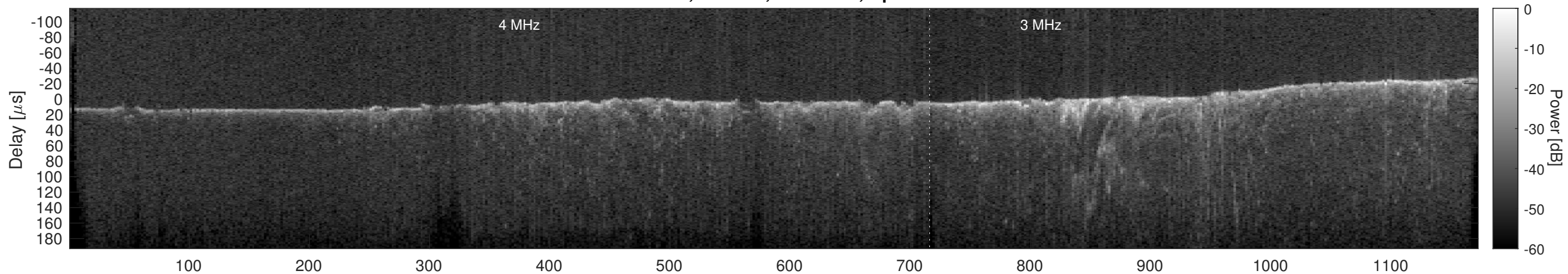
Orbit 17702, Cluttergram
