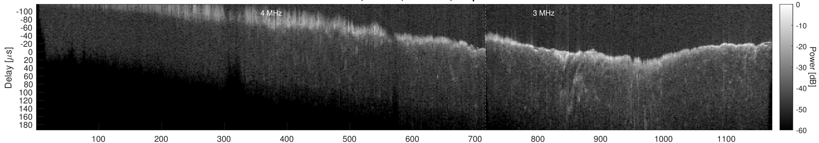
Orbit 17702, Window, Channel 2, Optimized
