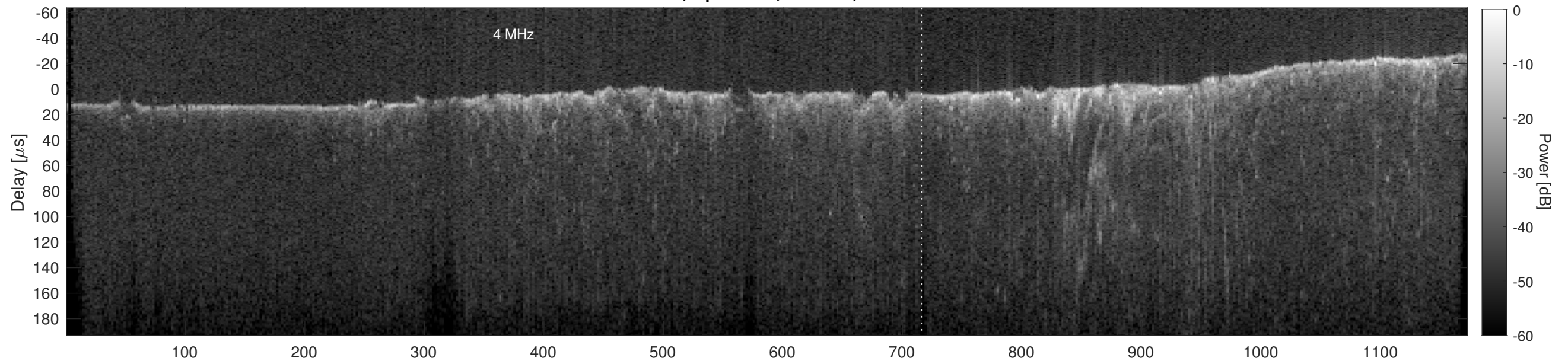
Orbit 17702, Cluttergram
