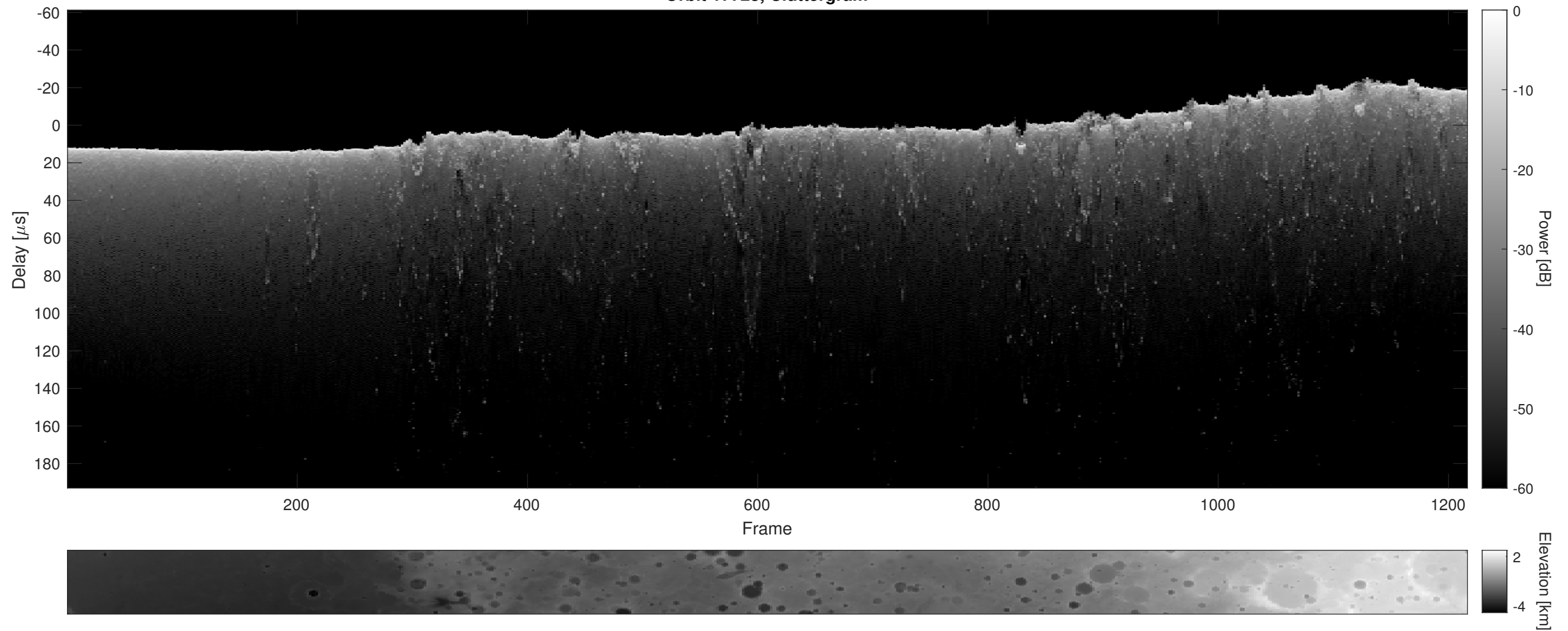
Orbit 17723, Cluttergram
