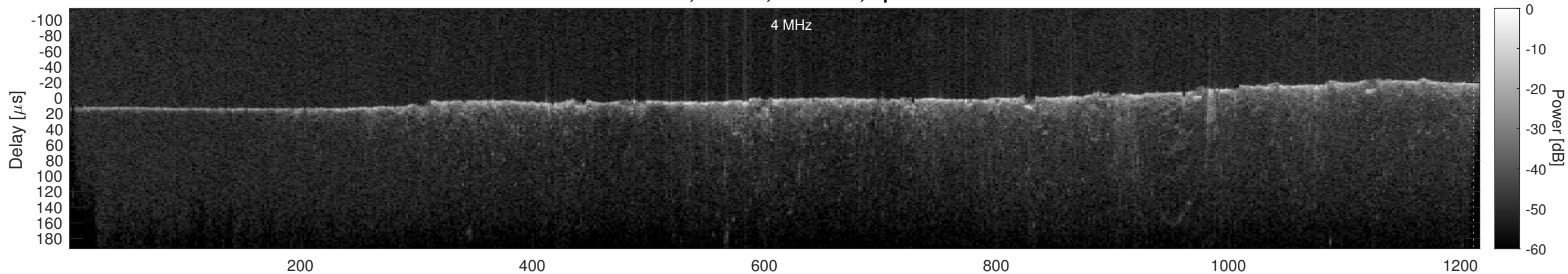
Orbit 17723, Cluttergram
