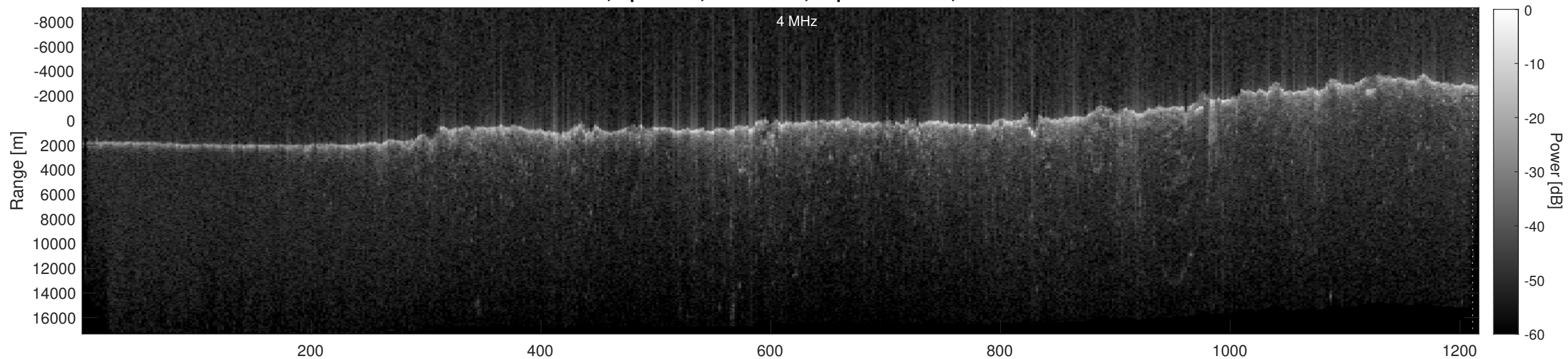
Orbit 17723, Depth-Corrected Cluttergram
