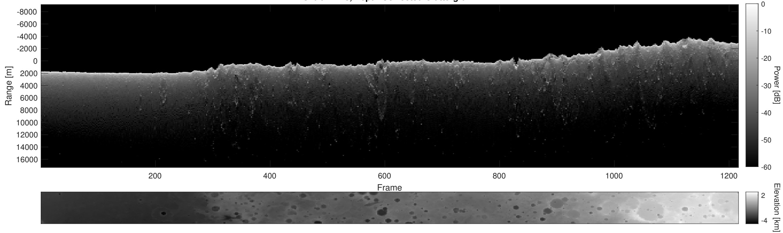
Orbit 17723, Depth-Corrected Cluttergram
