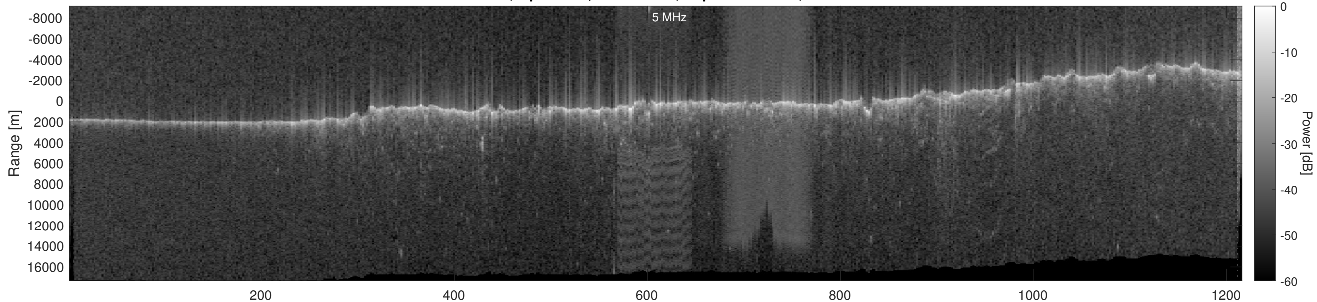
Orbit 17723, Optimized, No Window, Depth-Corrected, Channel 2
