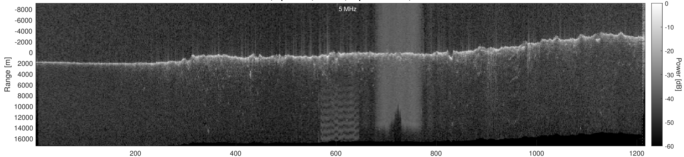
Orbit 17723, Optimized, Window, Depth-Corrected, Channel 2
