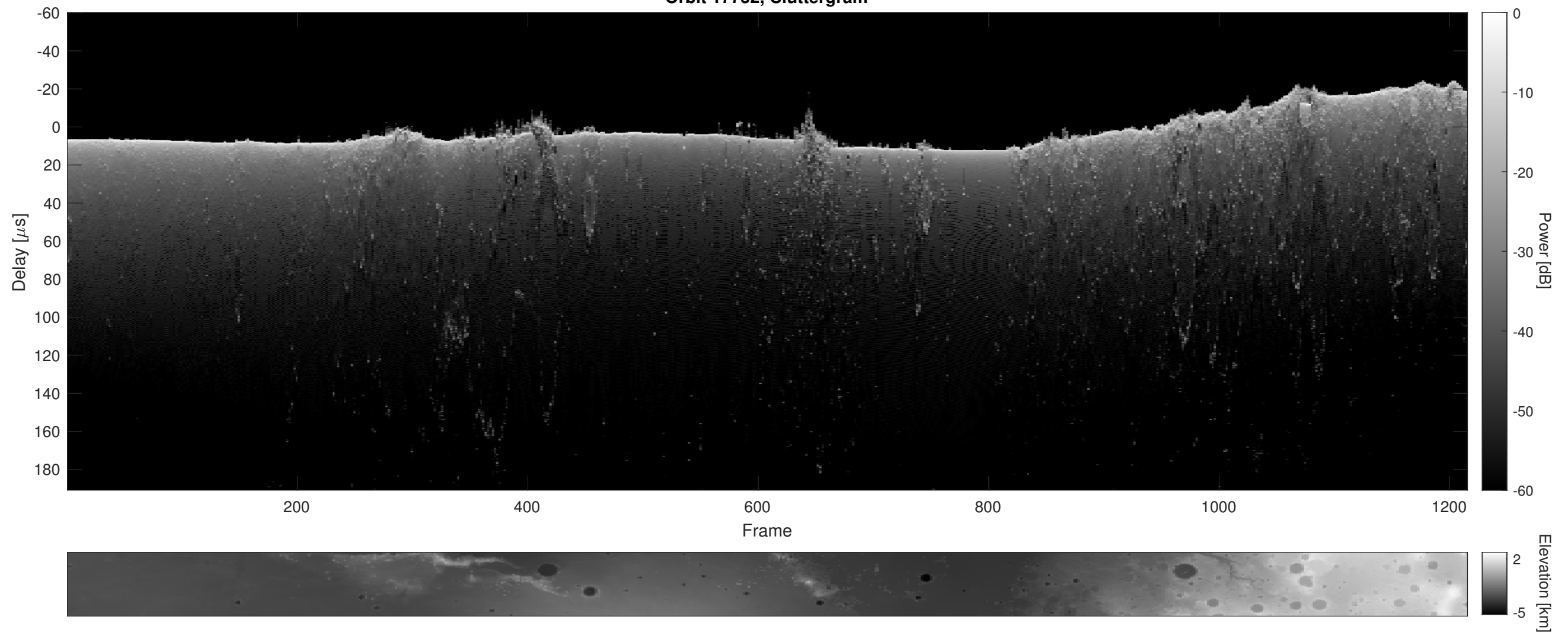
Orbit 17732, Cluttergram
