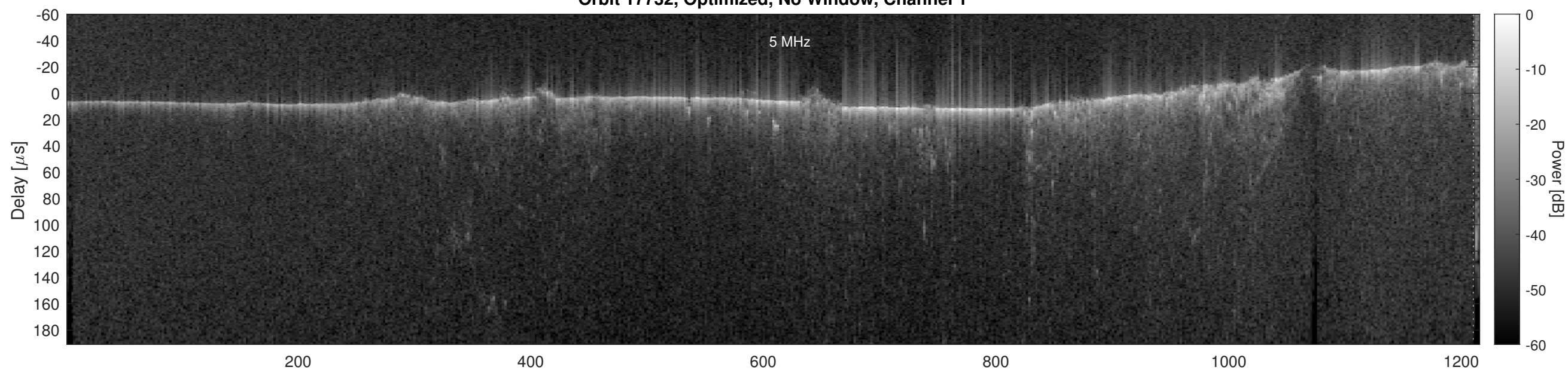
Orbit 17732, Optimized, No Window, Channel 2
