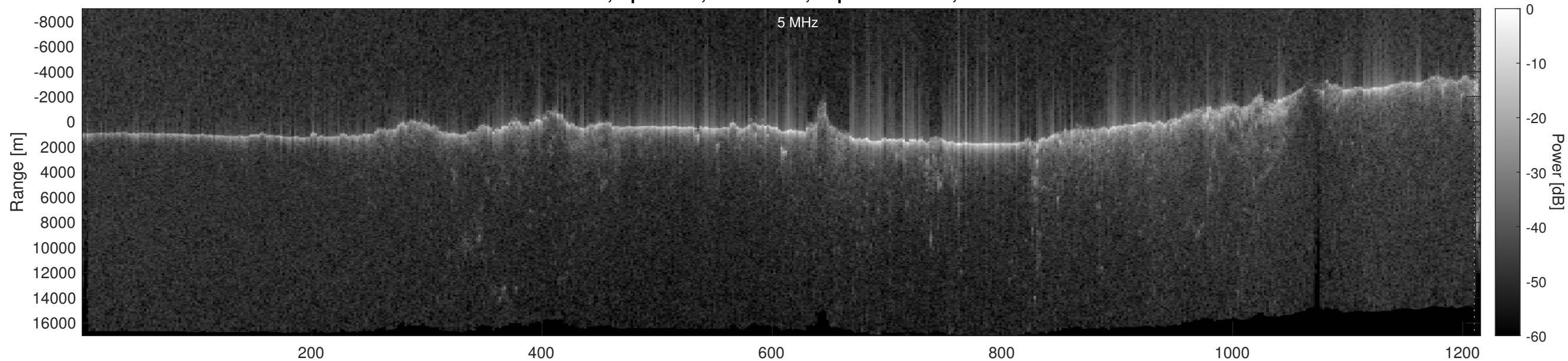
Orbit 17732, Optimized, No Window, Depth-Corrected, Channel 2
