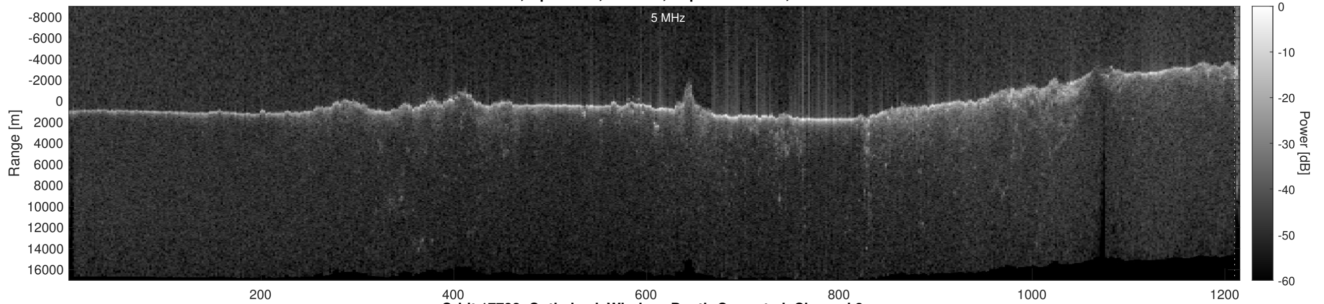
Orbit 17732, Optimized, Window, Depth-Corrected, Channel 2
