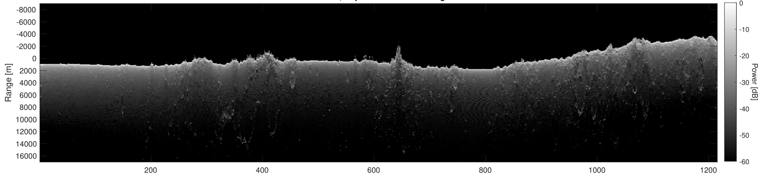
Orbit 17732, Depth-Corrected Cluttergram
