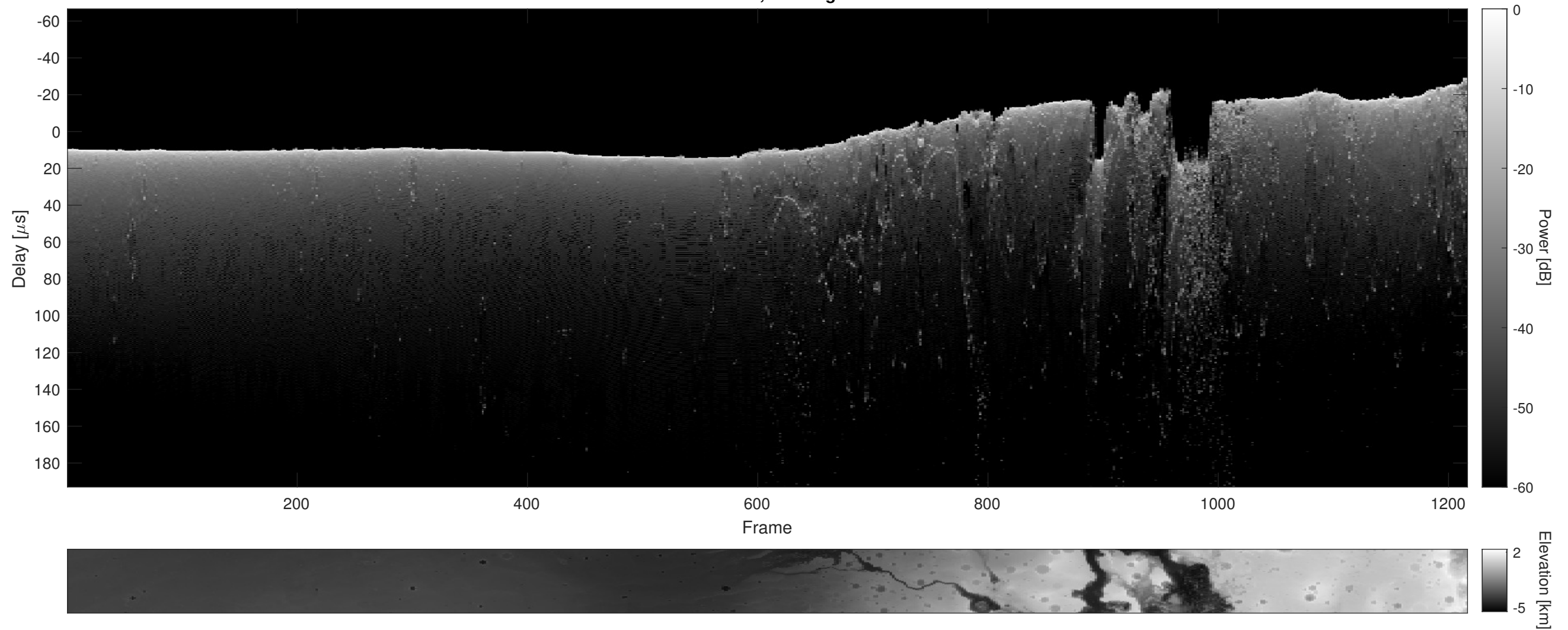
Orbit 17734, Cluttergram
