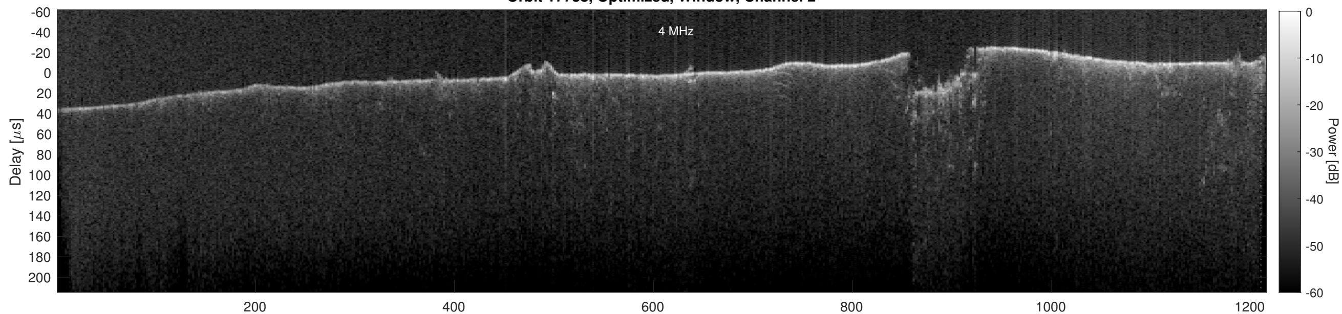
Orbit 17738, Cluttergram
