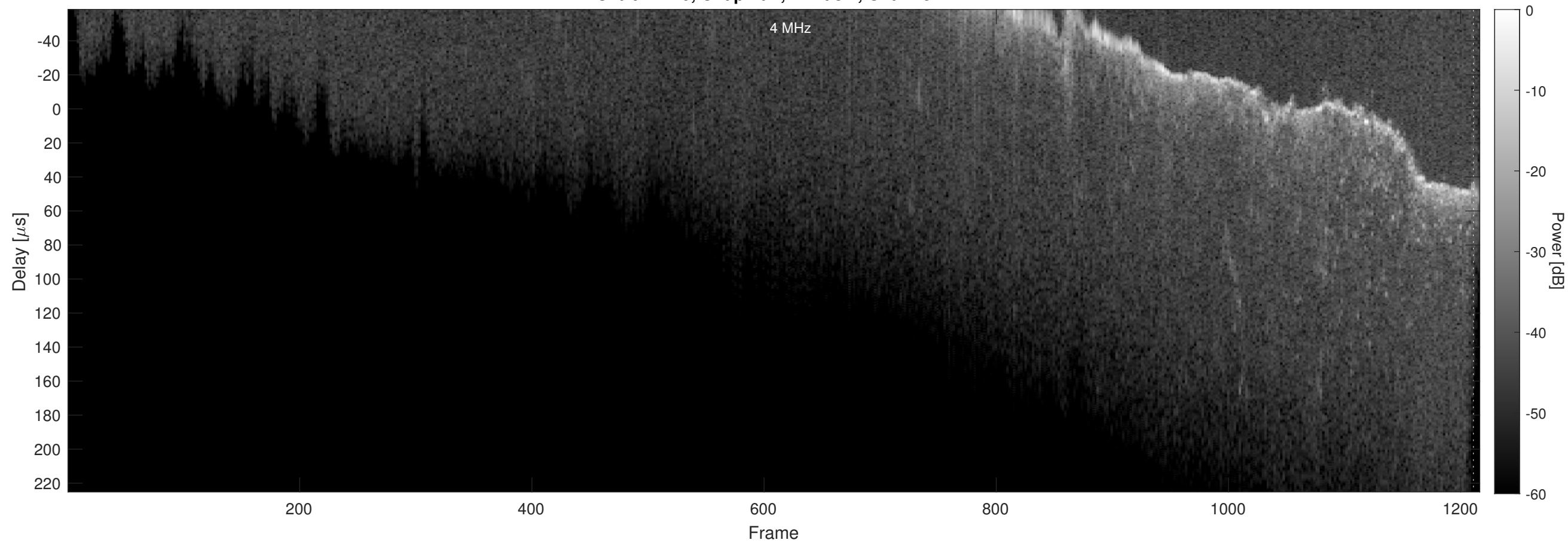
Orbit 17740, Chapman, Window, Channel 2
