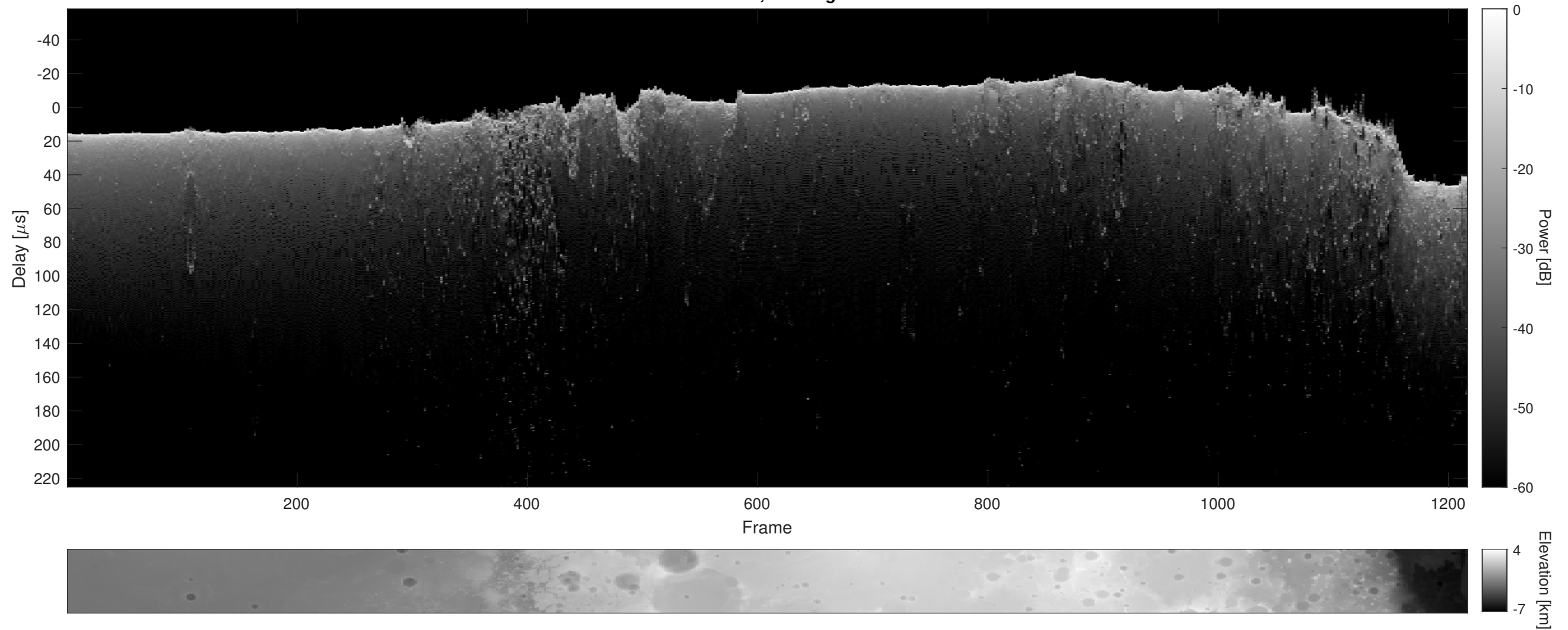
Orbit 17740, Cluttergram
