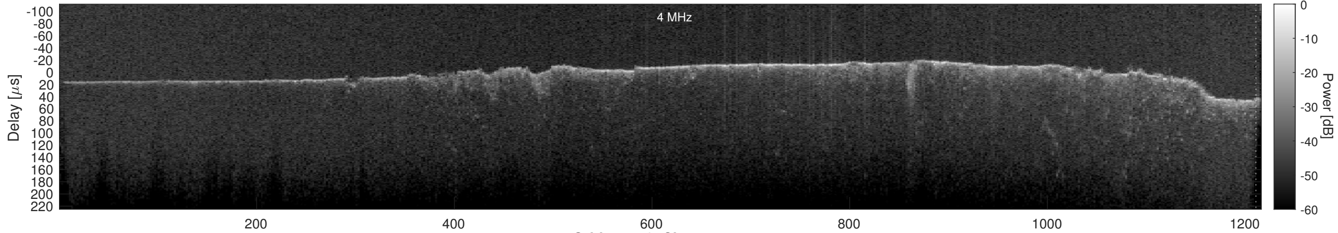
Orbit 17740, Cluttergram
