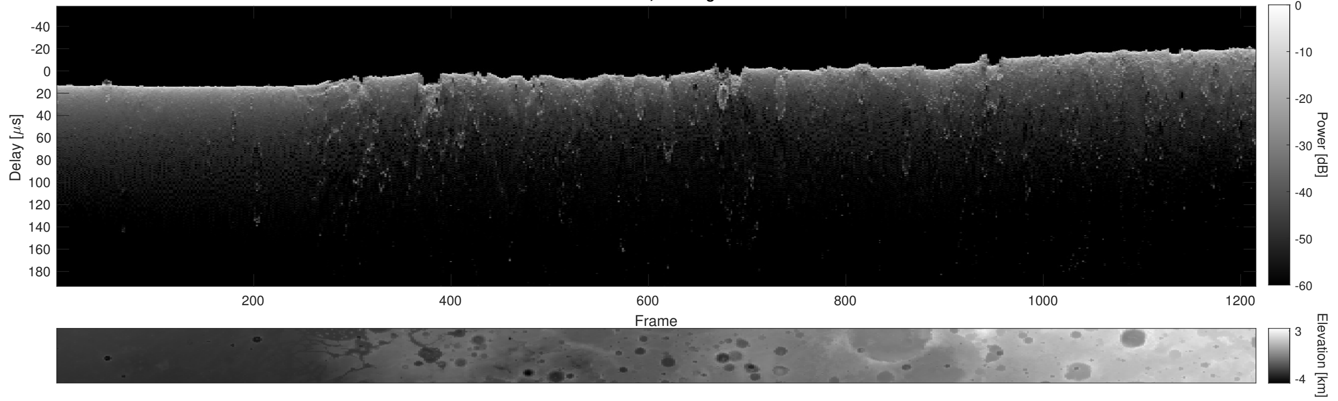
Orbit 17744, Cluttergram
