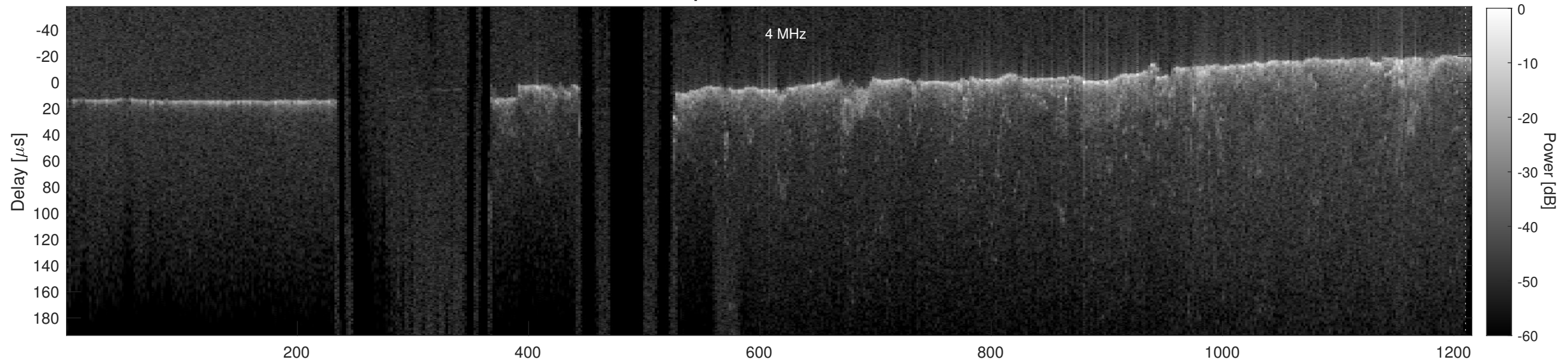
Orbit 17744, Cluttergram
