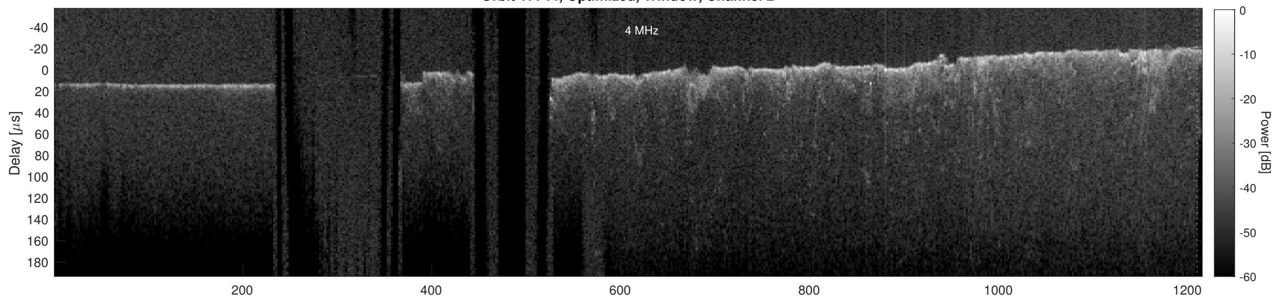
Orbit 17744, Cluttergram
