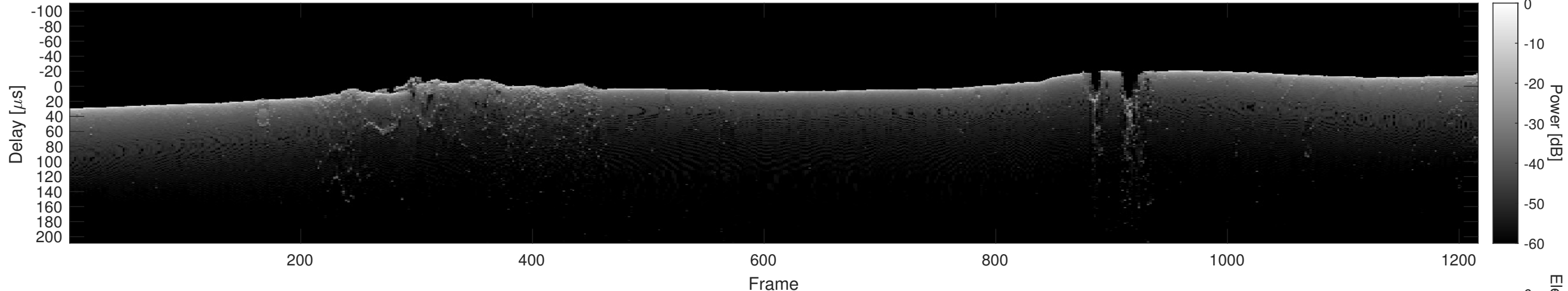
Orbit 17752, Cluttergram
