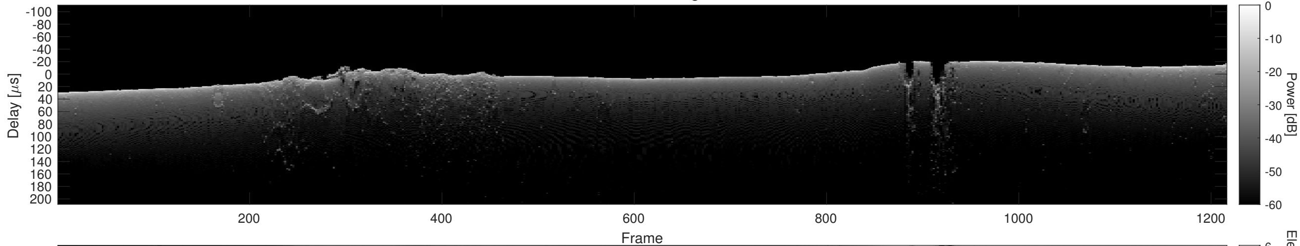
Orbit 17752, Cluttergram
