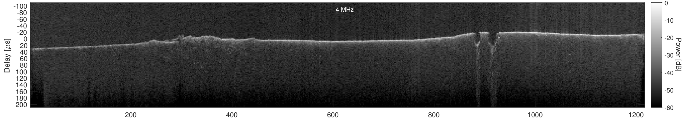
Orbit 17752, Cluttergram
