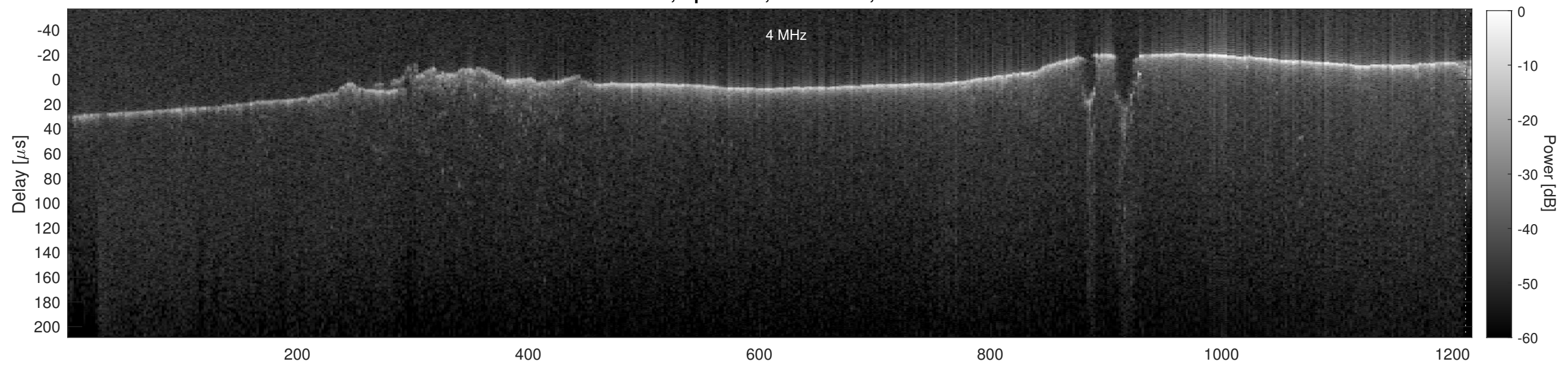
Orbit 17752, Cluttergram
