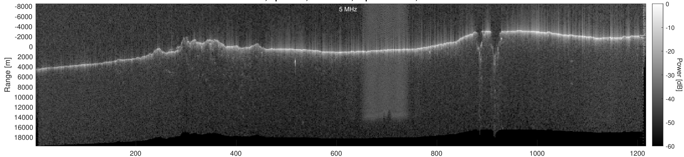
Orbit 17752, Optimized, No Window, Depth-Corrected, Channel 2
