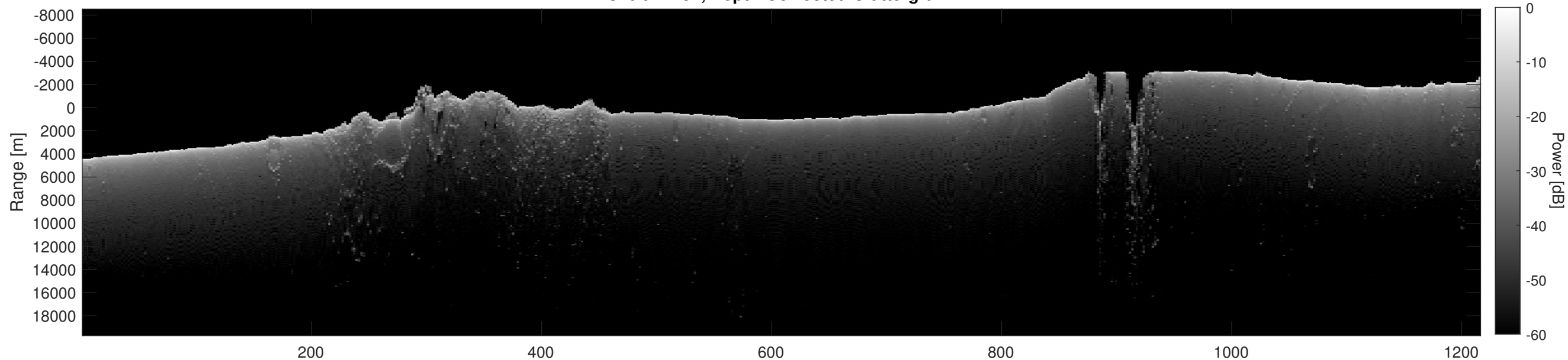
Orbit 17752, Depth-Corrected Cluttergram
