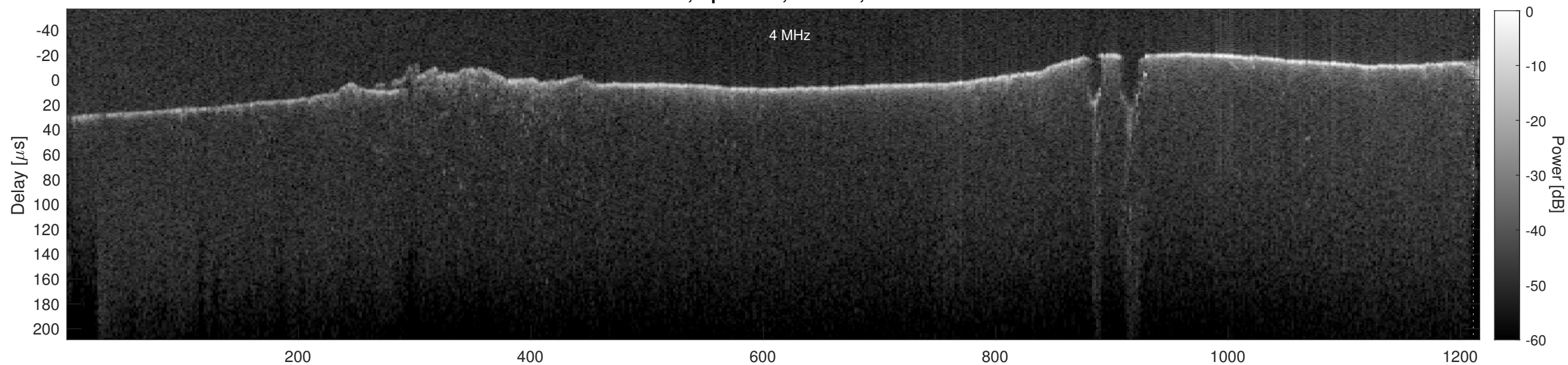
Orbit 17752, Cluttergram
