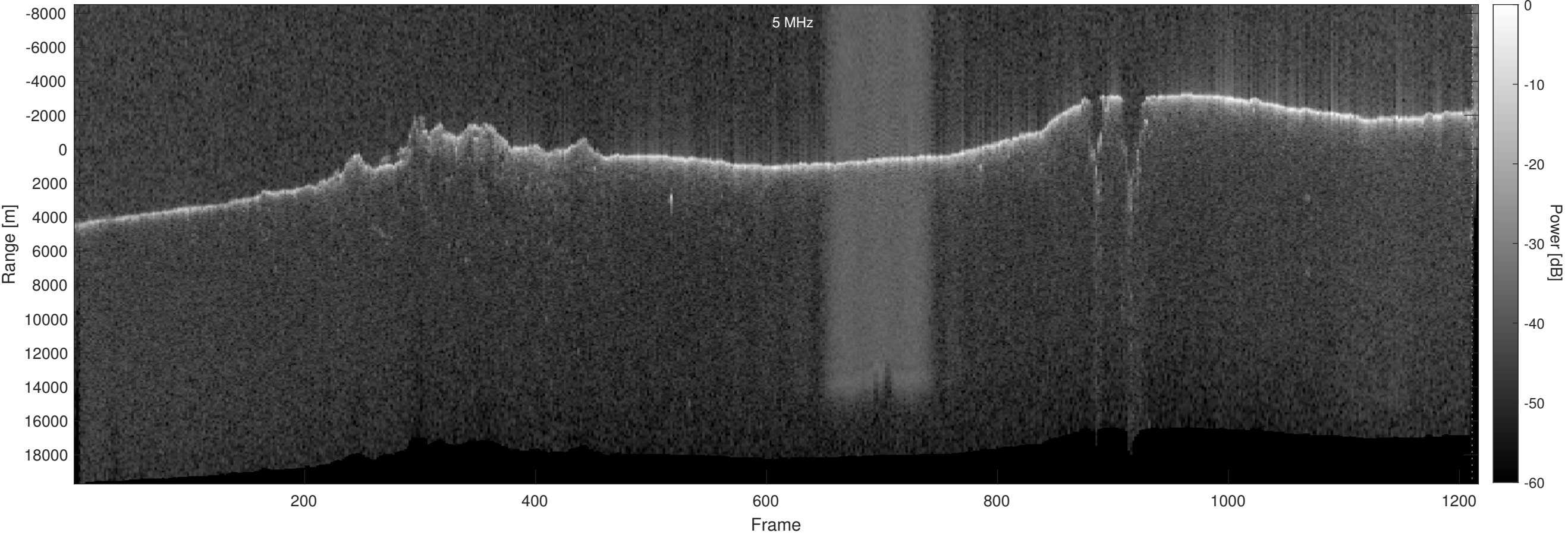
Orbit 17752, Optimized, Window, Depth-Corrected, Channel 2
