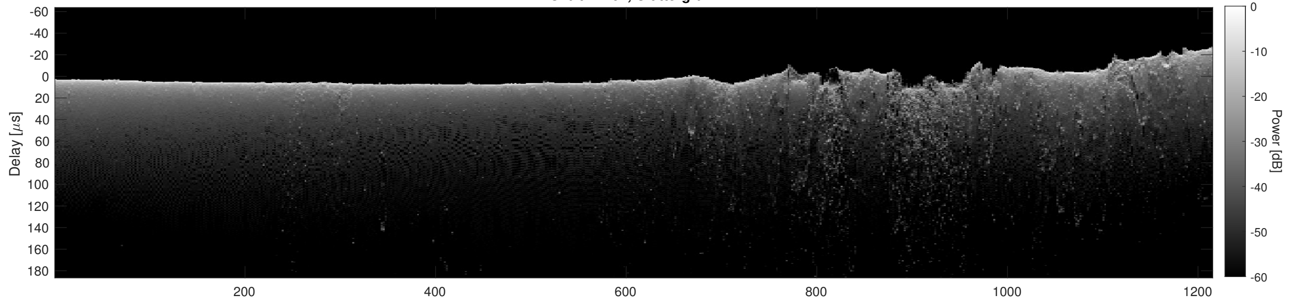
Orbit 17762, Cluttergram
