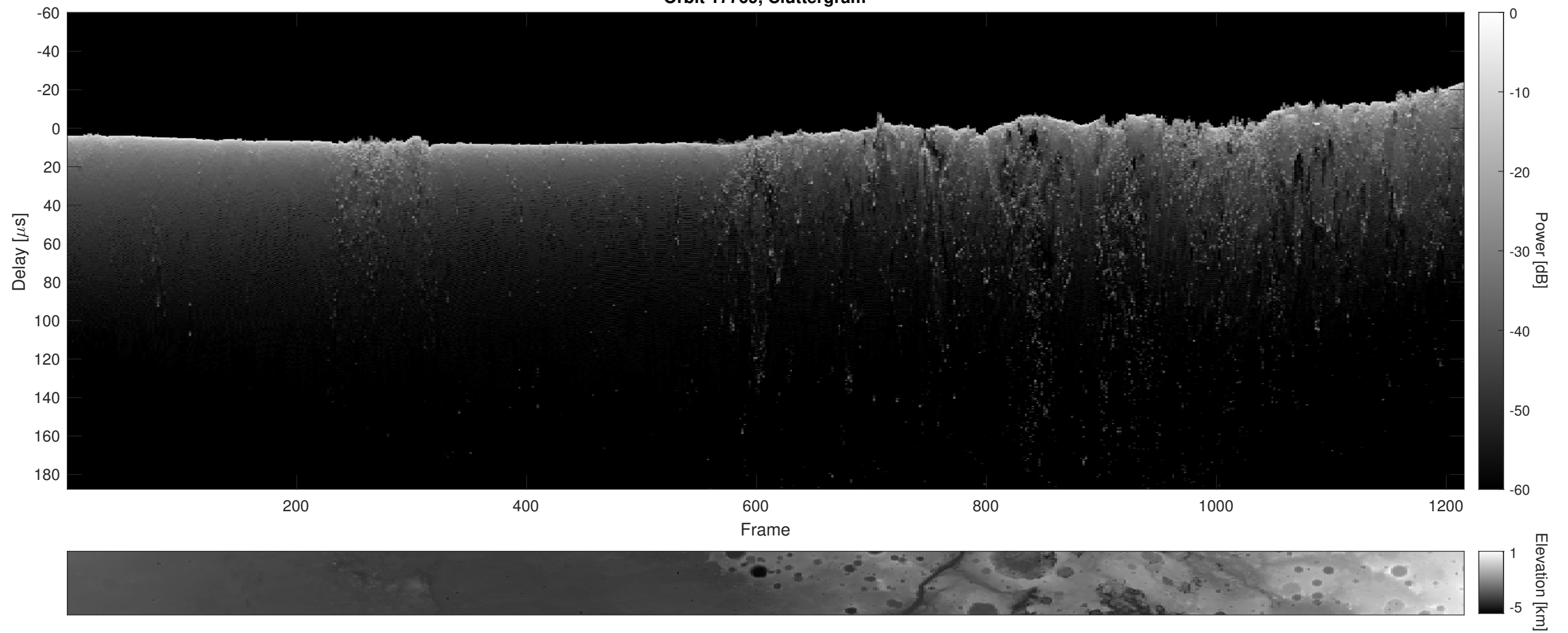
Orbit 17769, Cluttergram
