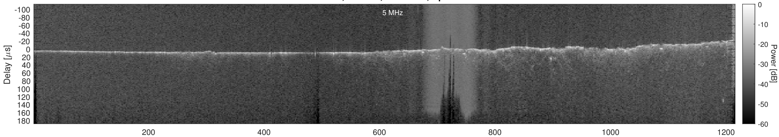
Orbit 17769, Cluttergram
