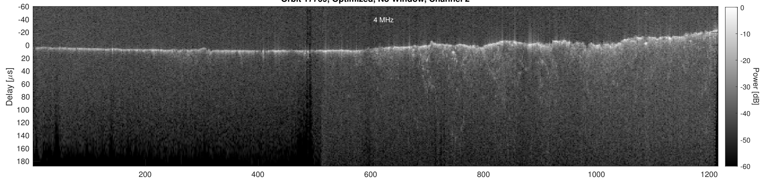
Orbit 17769, Cluttergram
