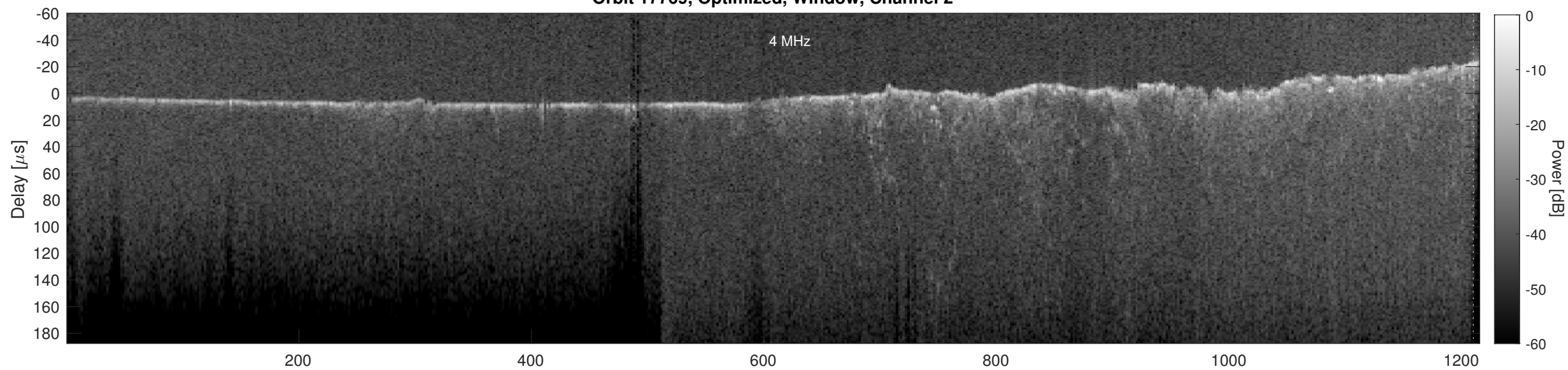
Orbit 17769, Cluttergram
