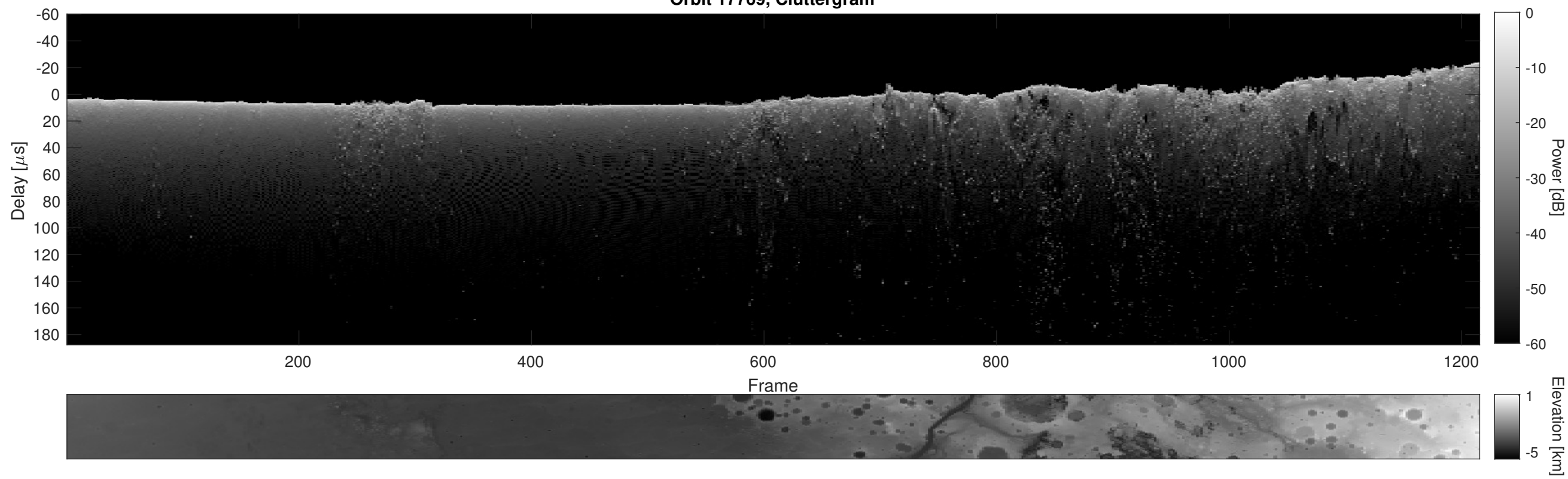
Orbit 17769, Cluttergram
