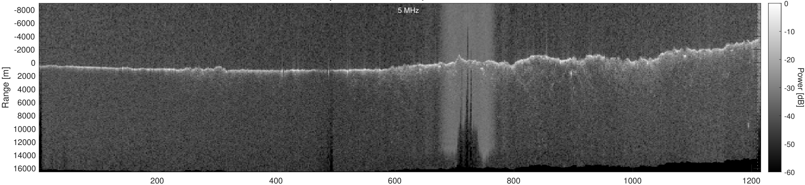
Orbit 17769, Optimized, Window, Depth-Corrected, Channel 2
