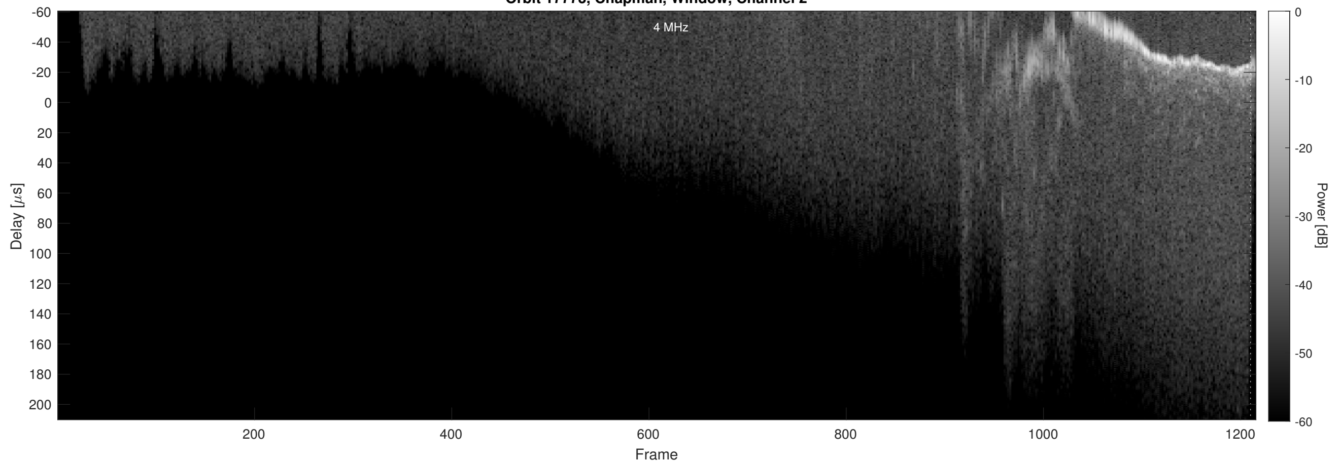
Orbit 17773, Chapman, Window, Channel 2
