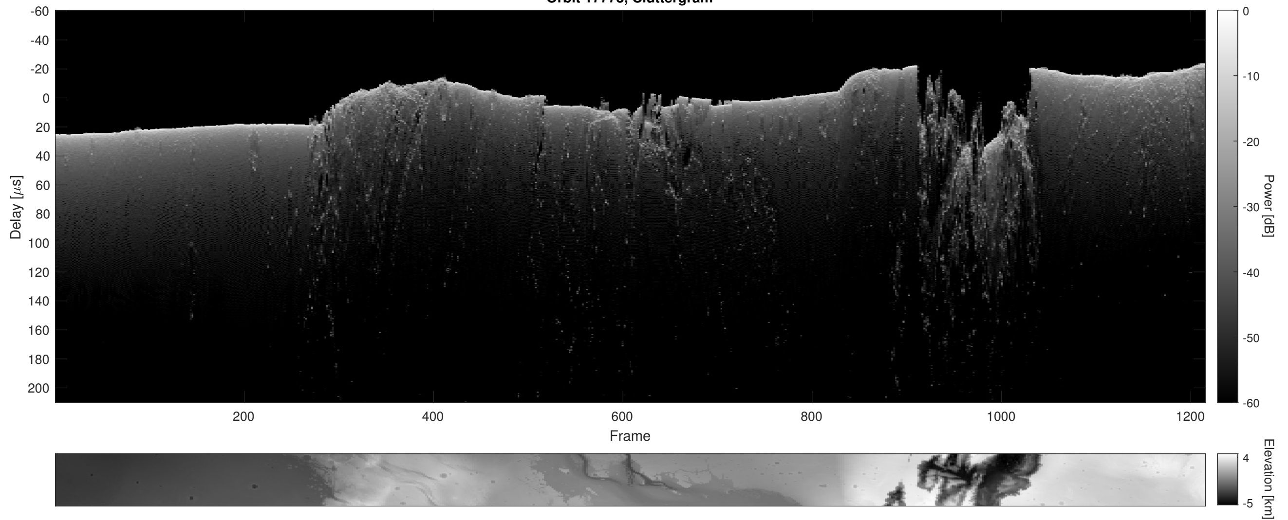
Orbit 17773, Cluttergram
