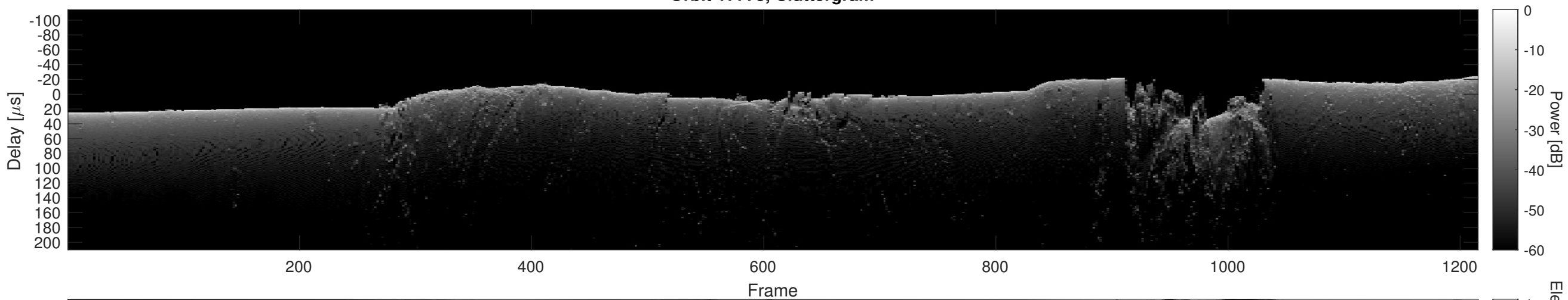
Orbit 17773, Cluttergram
