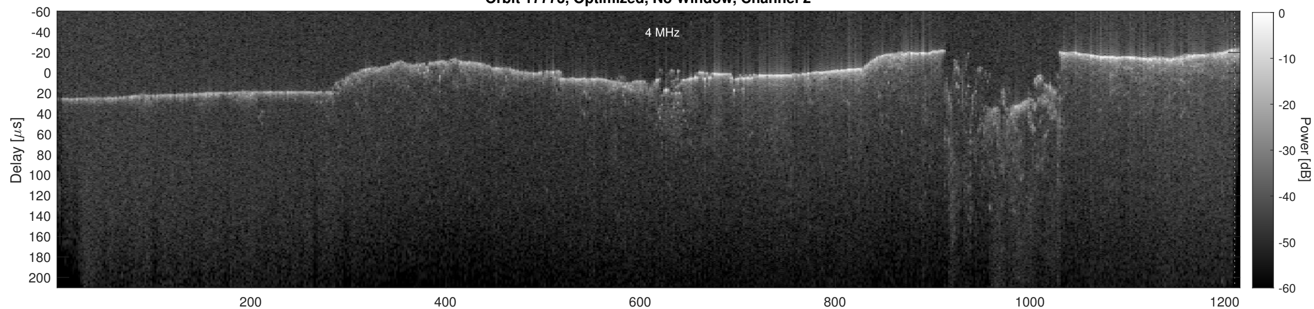
Orbit 17773, Cluttergram
