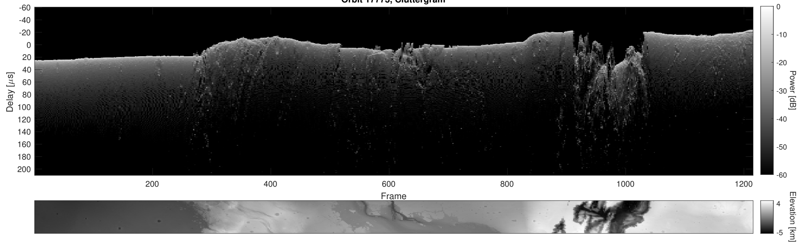
Orbit 17773, Cluttergram
