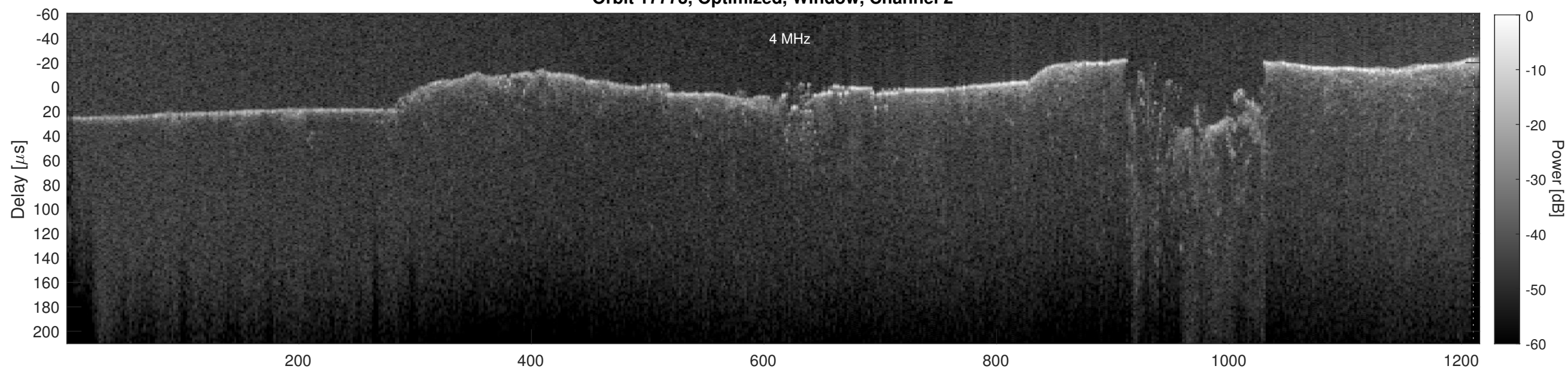
Orbit 17773, Cluttergram
