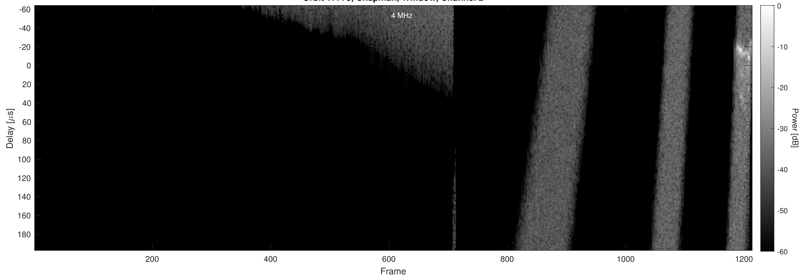
Orbit 17775, Chapman, Window, Channel 2
