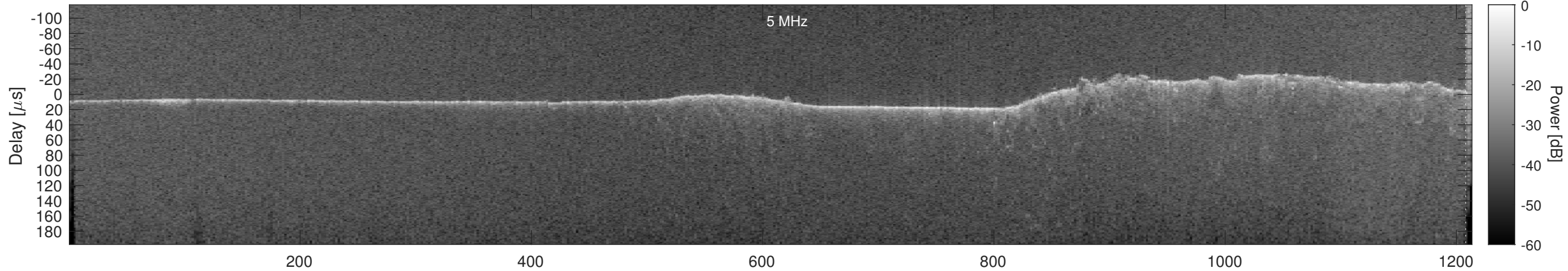
Orbit 17775, Cluttergram
