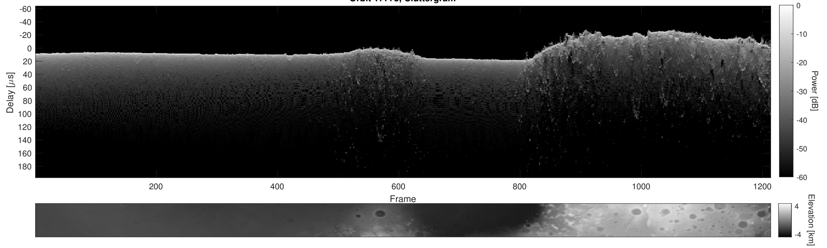
Orbit 17775, Cluttergram
