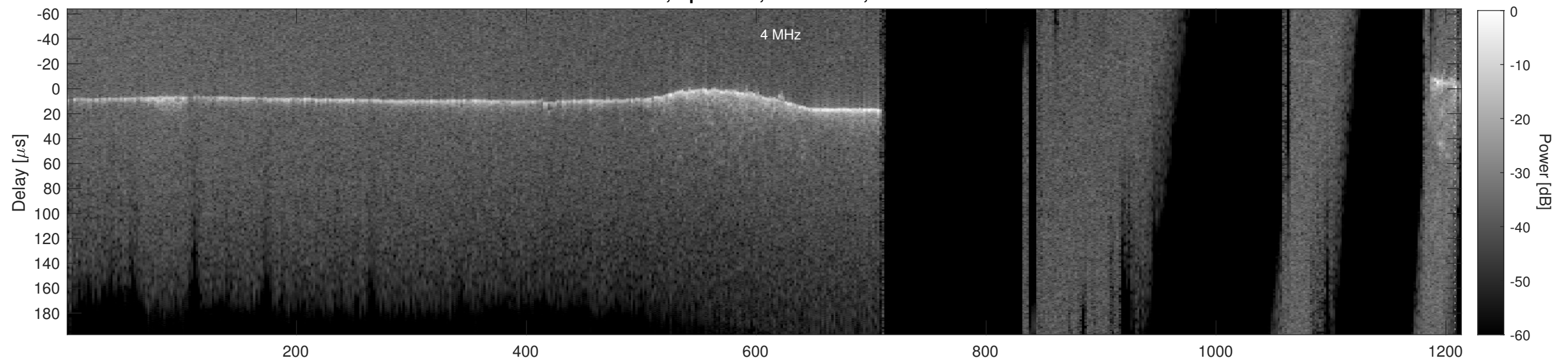
Orbit 17775, Cluttergram
