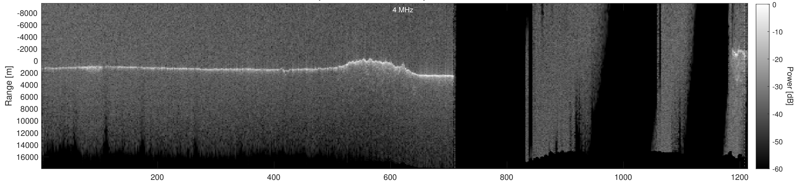
Orbit 17775, Depth-Corrected Cluttergram
