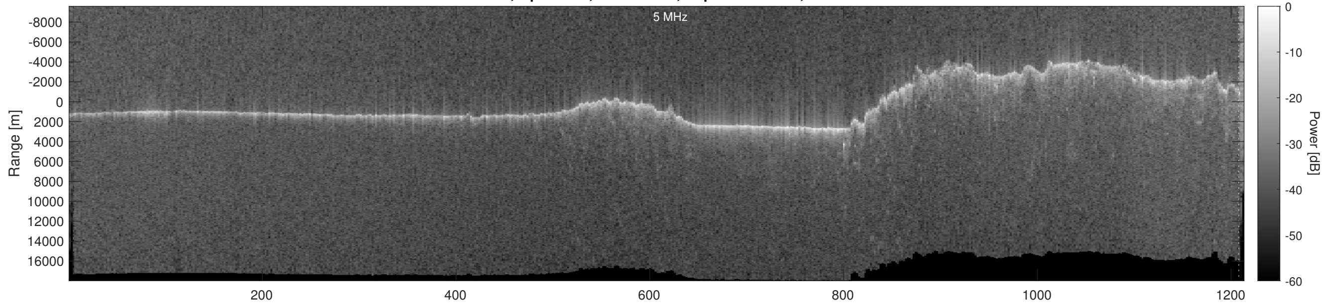
Orbit 17775, Optimized, No Window, Depth-Corrected, Channel 2
