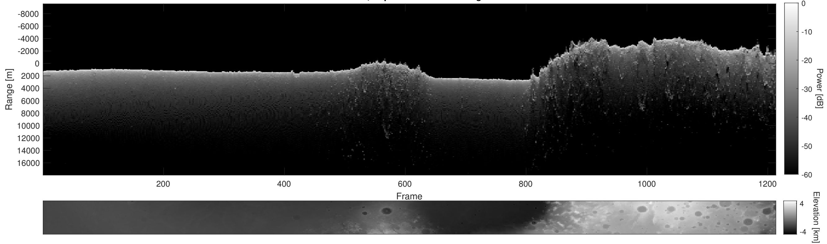
Orbit 17775, Depth-Corrected Cluttergram
