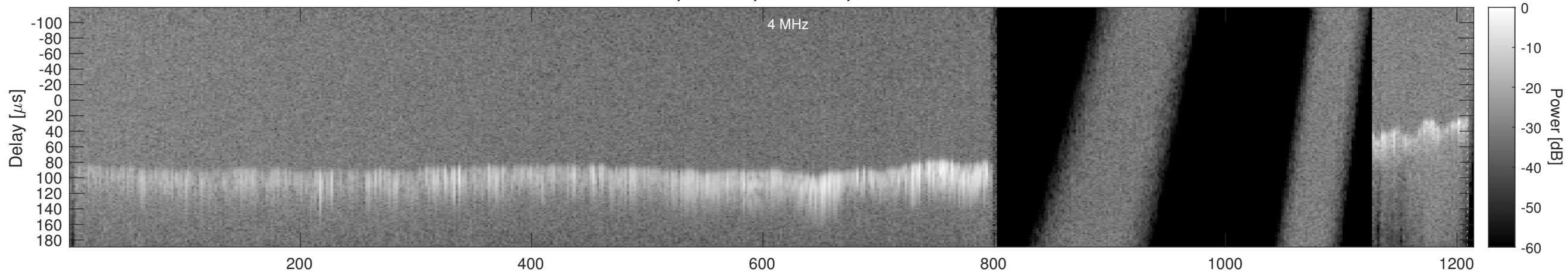
Orbit 17802, Window, Channel 2, Chapman
