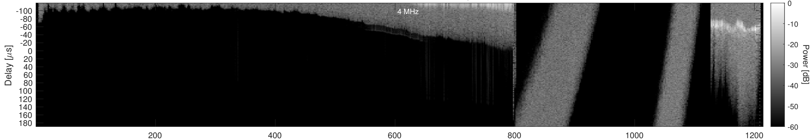
Orbit 17802, Window, Channel 2, Optimized
