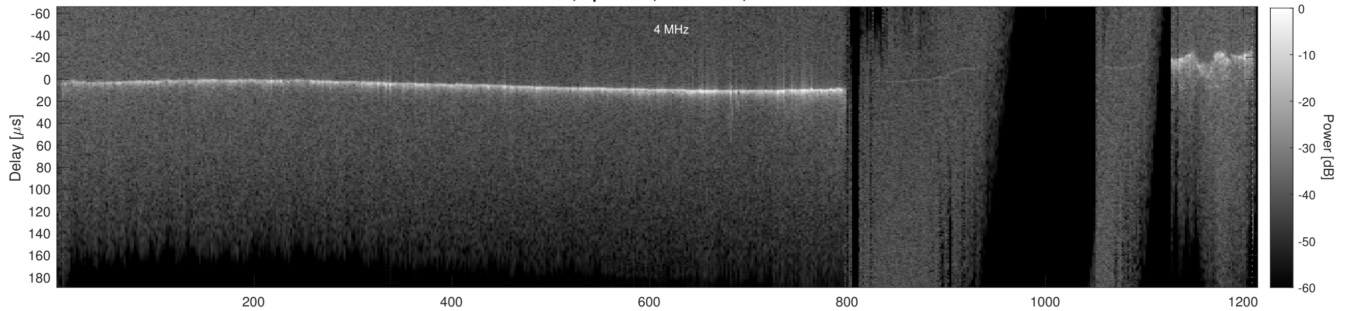
Orbit 17802, Cluttergram
