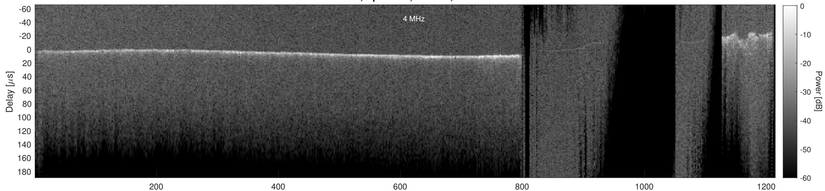
Orbit 17802, Cluttergram
