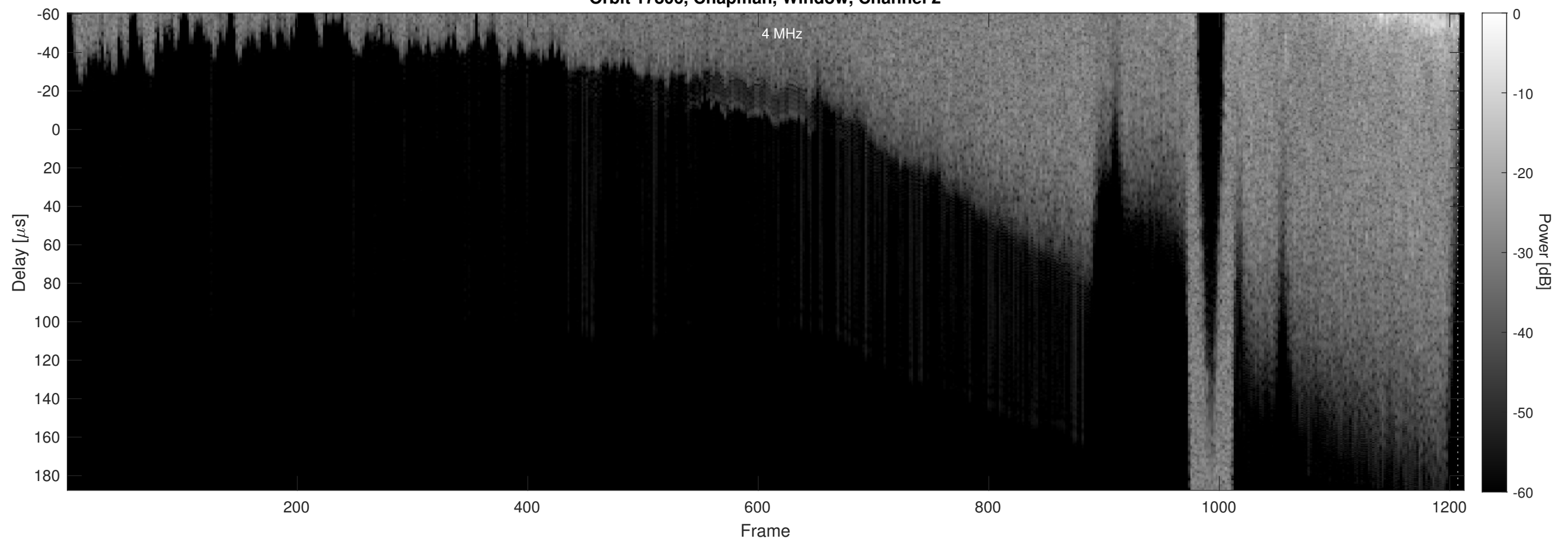
Orbit 17806, Chapman, Window, Channel 2
