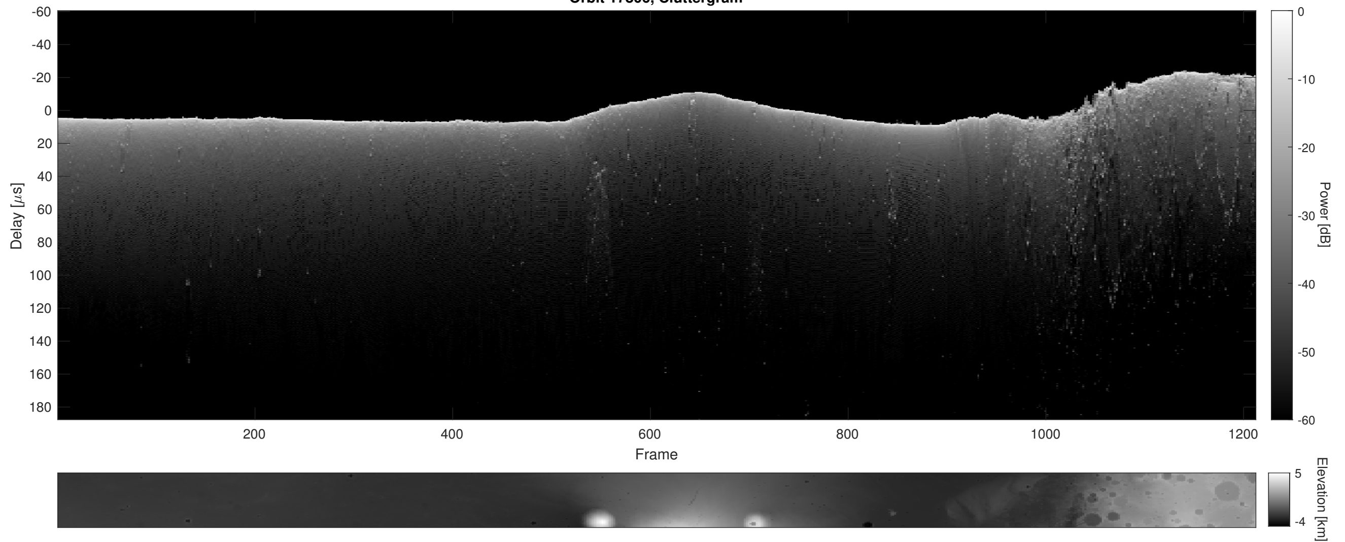
Orbit 17806, Cluttergram
