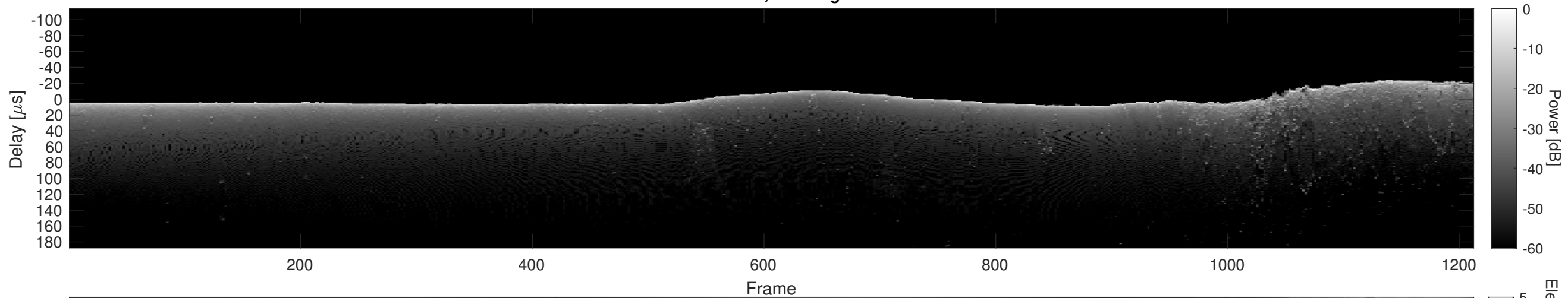
Orbit 17806, Cluttergram
