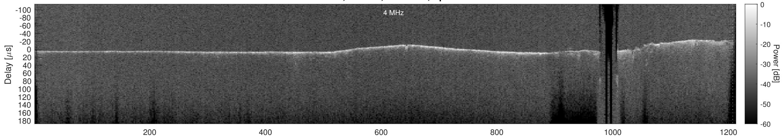
Orbit 17806, Cluttergram
