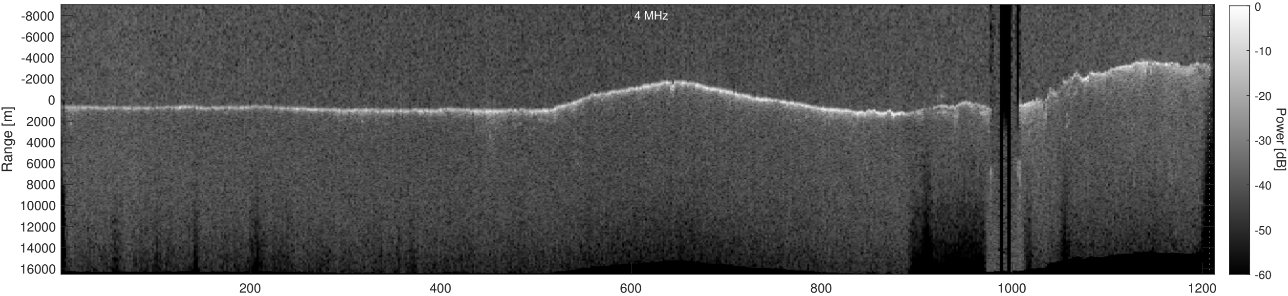
Orbit 17806, Depth-Corrected Cluttergram
