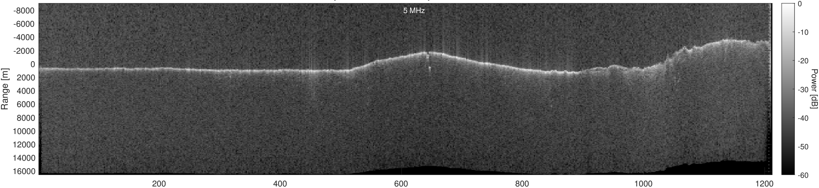
Orbit 17806, Optimized, Window, Depth-Corrected, Channel 2
