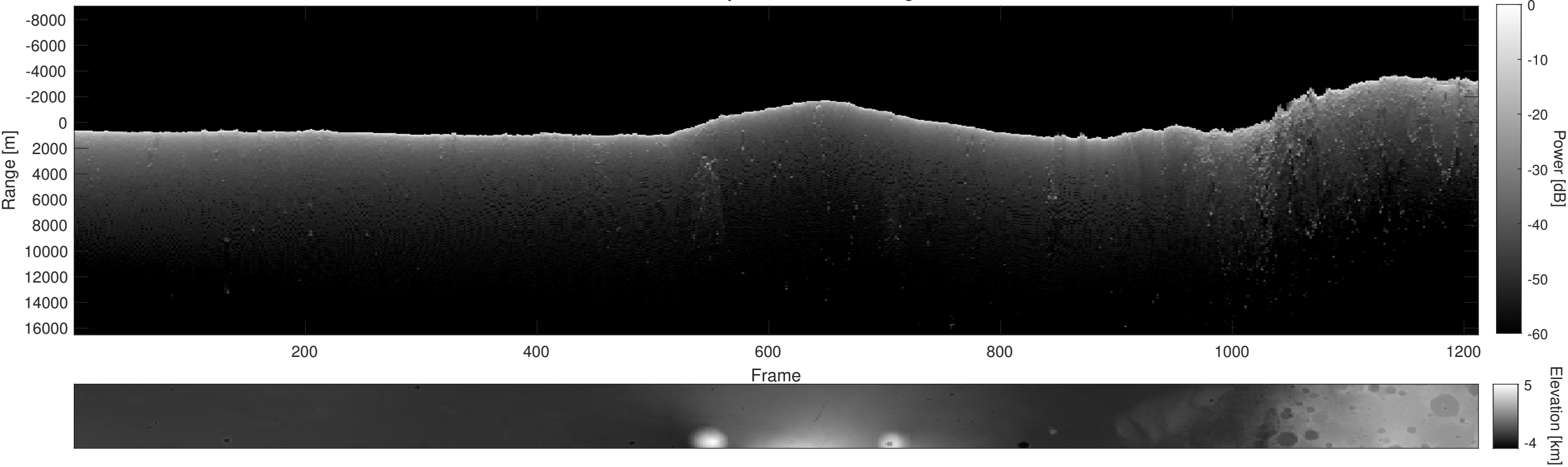
Orbit 17806, Depth-Corrected Cluttergram
