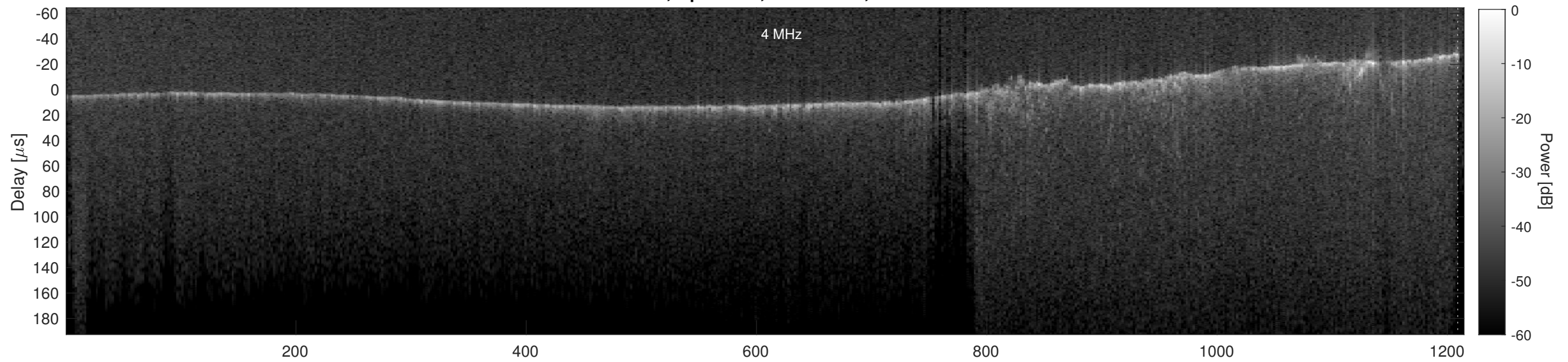
Orbit 17810, Cluttergram
