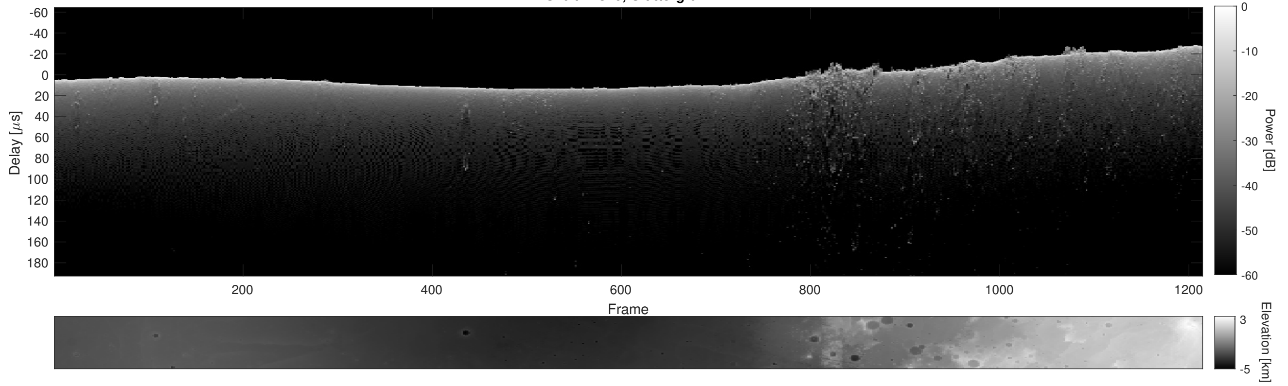
Orbit 17810, Cluttergram
