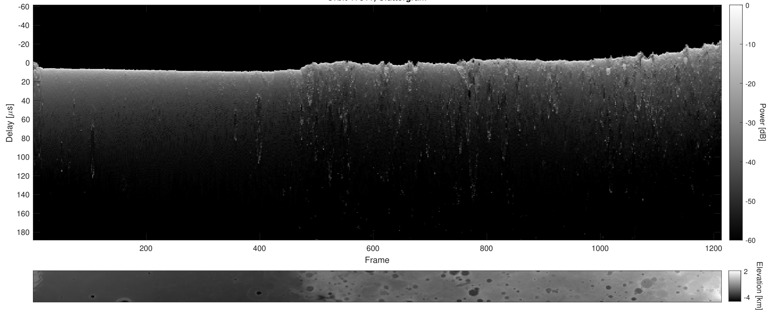
Orbit 17811, Cluttergram
