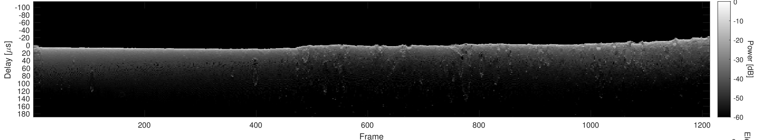
Orbit 17811, Cluttergram
